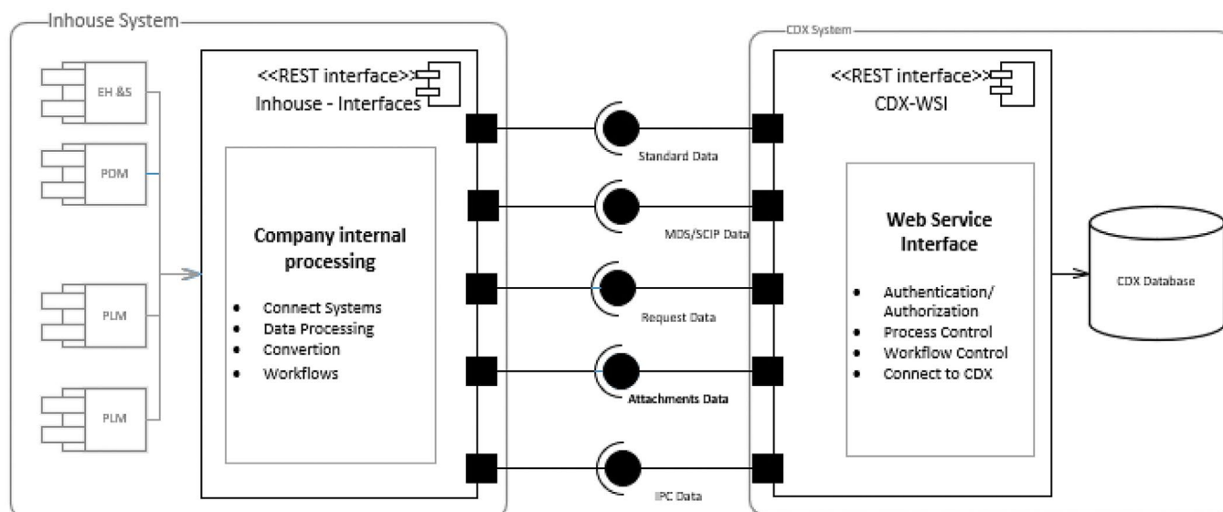
Figure 1. Function Chart of the CDX-WSI
